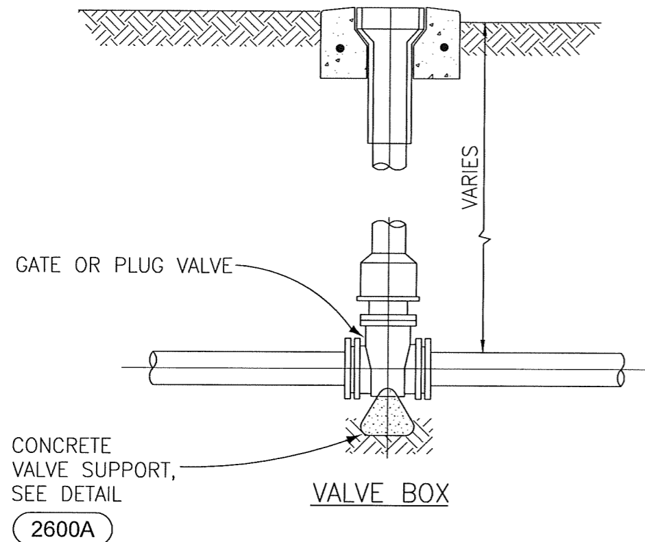
BURIED VALVE NOT TO SCALE
