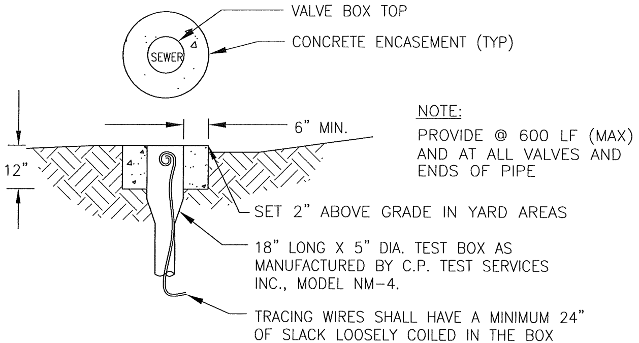
TRACER WIRE DETAIL NOT TO SCALE
